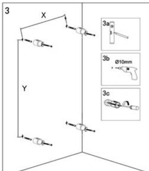
Figure 4 | Fixing the wall brackets
