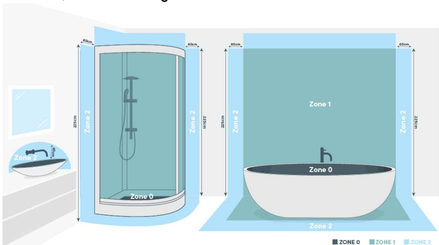
Figure 1 | Bathroom installation zones
